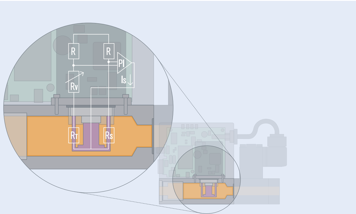
Functional schematic of Inline sensor
