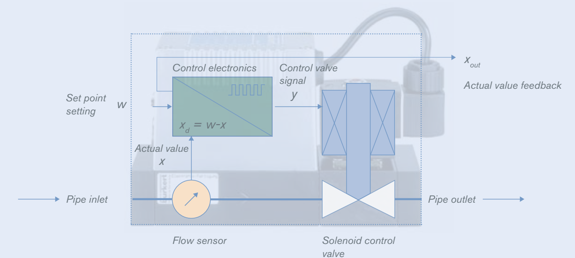
Basic principle closed control loop
